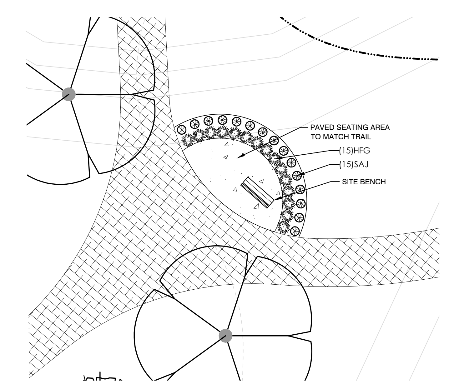
POCKET PARK - 2 SCALE: 1" = 10'
